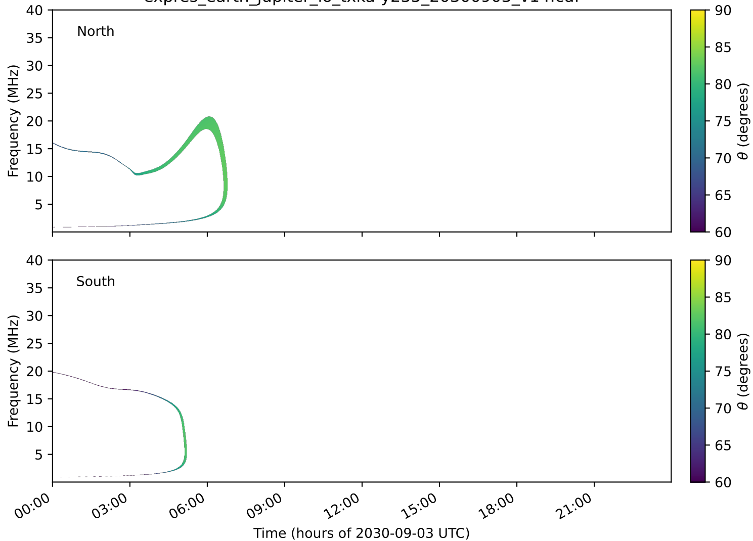
expres_earth_jupiter_io_txka-y235_20300903_v14.cdf
