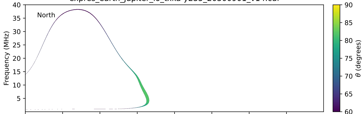
expres_earth_jupiter_io_txka-y235_20300901_v14.cdf
