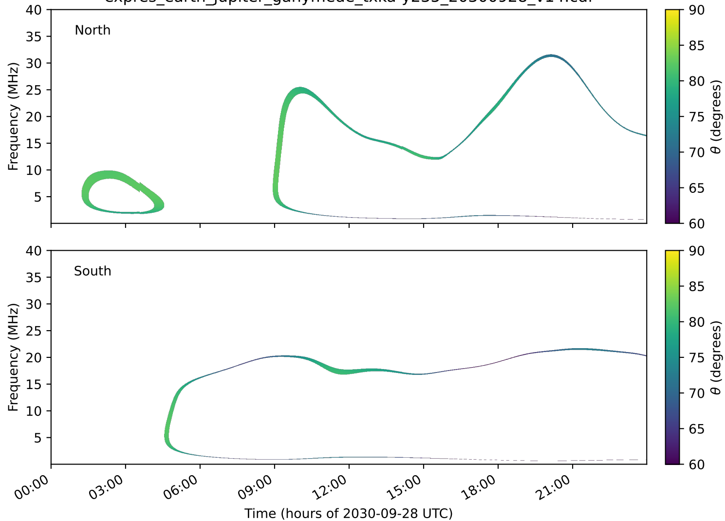
expres_earth_jupiter_ganymede_txka-y235_20300928_v14.cdf
