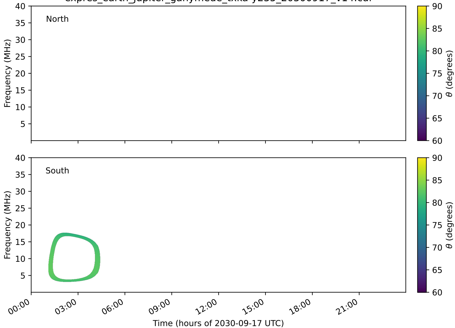
expres_earth_jupiter_ganymede_txka-y235_20300917_v14.cdf
