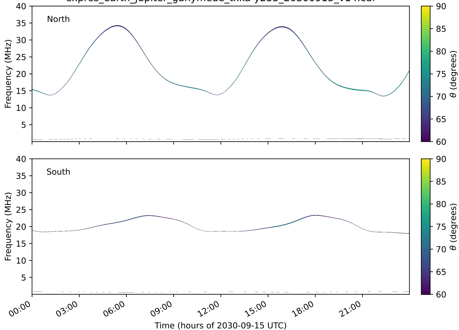
expres_earth_jupiter_ganymede_txka-y235_20300915_v14.cdf
