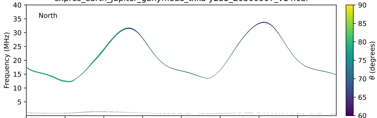
expres_earth_jupiter_ganymede_txka-y235_20300907_v14.cdf
