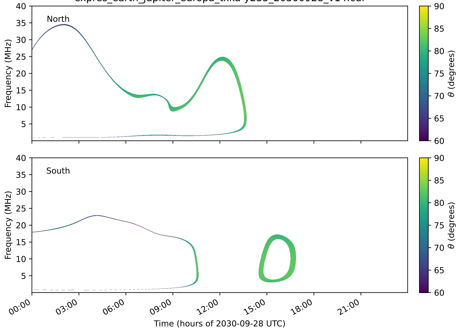
expres_earth_jupiter_europa_txka-y235_20300928_v14.cdf
