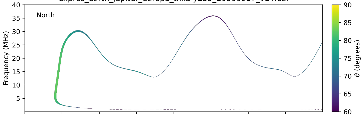
expres_earth_jupiter_europa_txka-y235_20300927_v14.cdf
