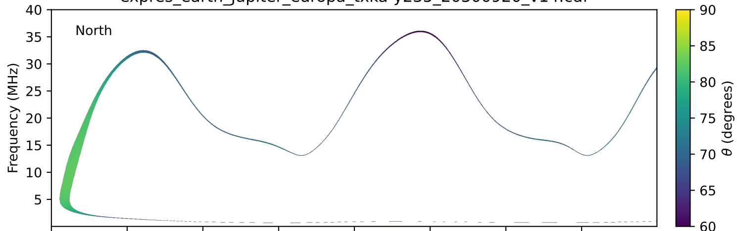
expres_earth_jupiter_europa_txka-y235_20300920_v14.cdf
