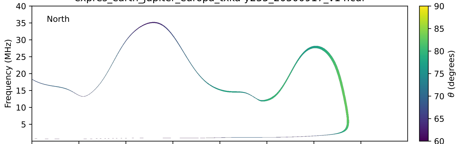
expres_earth_jupiter_europa_txka-y235_20300917_v14.cdf
