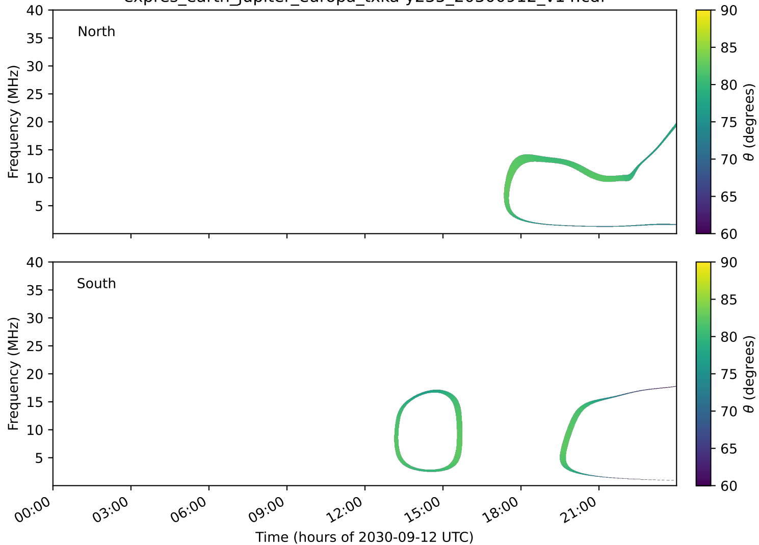
expres_earth_jupiter_europa_txka-y235_20300912_v14.cdf
