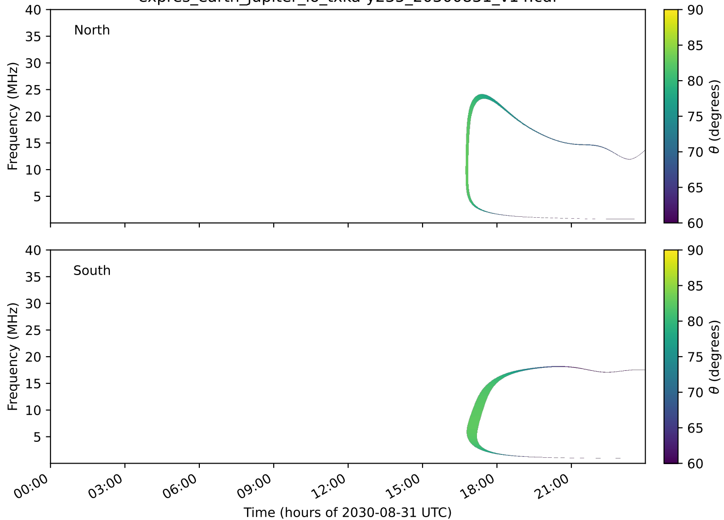
expres_earth_jupiter_io_txka-y235_20300831_v14.cdf
