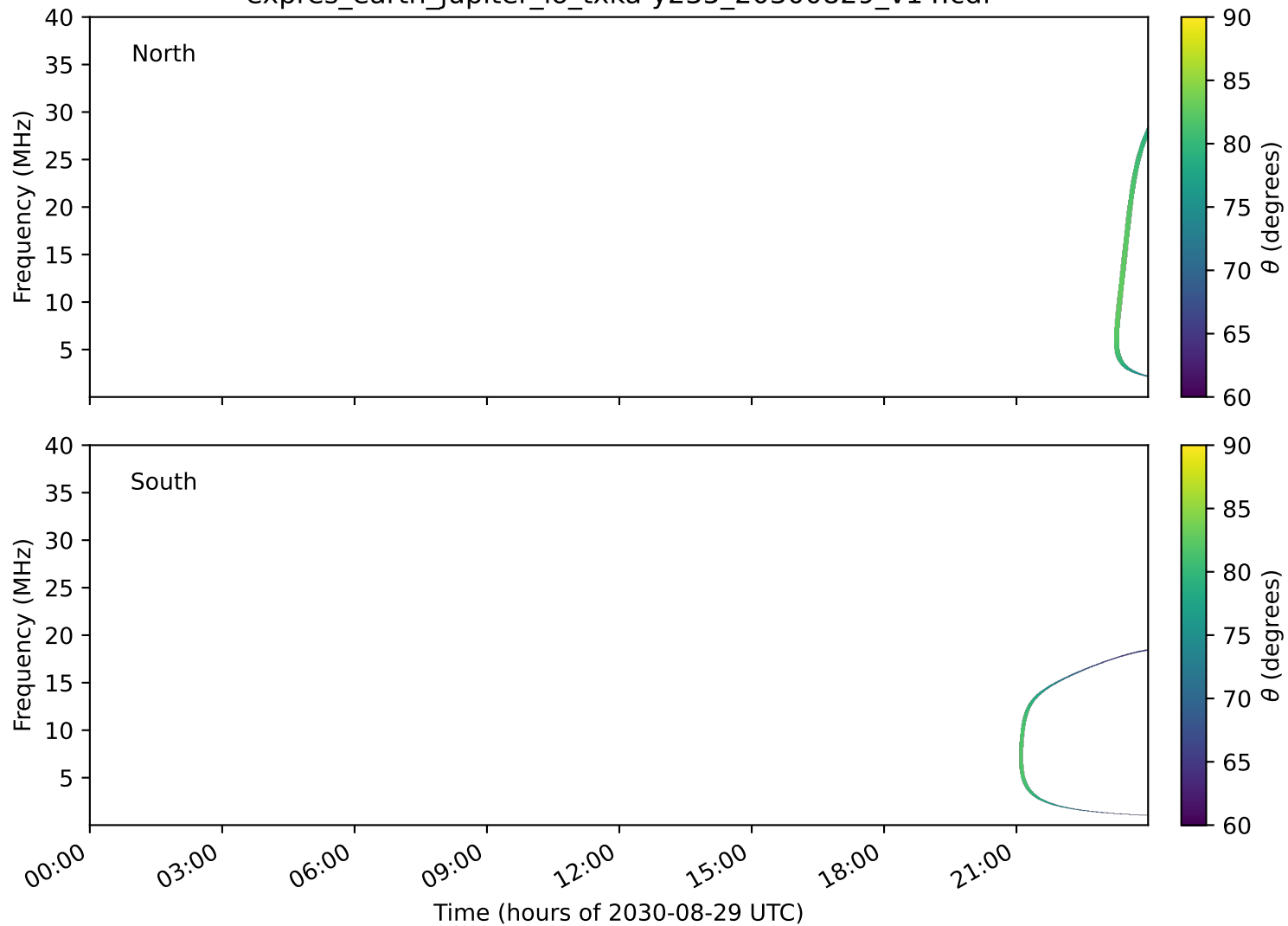
expres_earth_jupiter_io_txka-y235_20300829_v14.cdf
