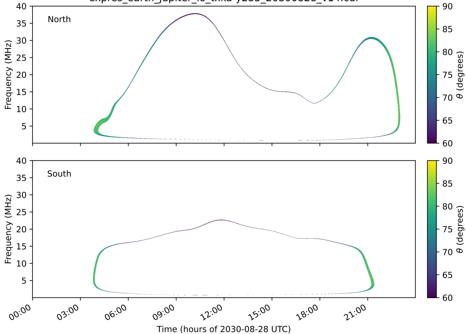
expres_earth_jupiter_io_txka-y235_20300828_v14.cdf
