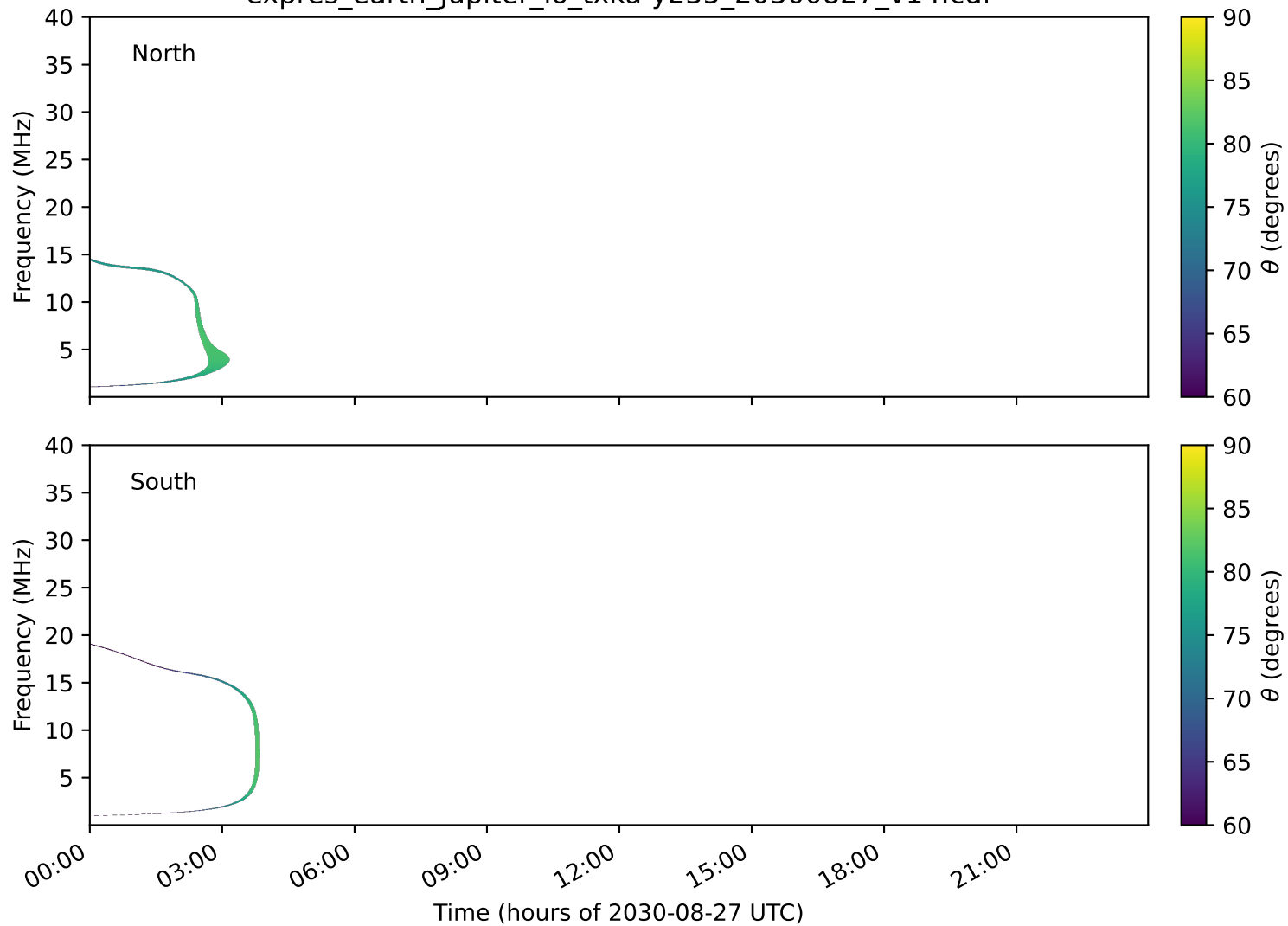
expres_earth_jupiter_io_txka-y235_20300827_v14.cdf
