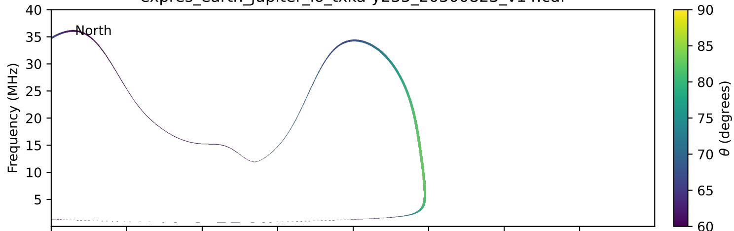
expres_earth_jupiter_io_txka-y235_20300823_v14.cdf
