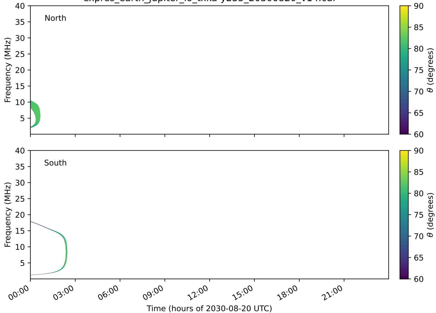
expres_earth_jupiter_io_txka-y235_20300820_v14.cdf
