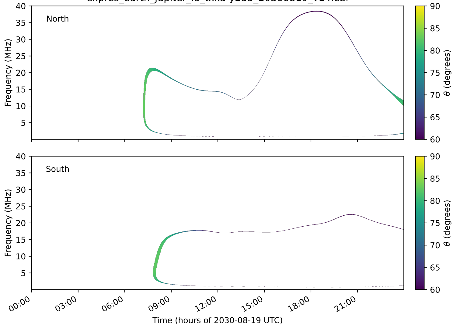
expres_earth_jupiter_io_txka-y235_20300819_v14.cdf
