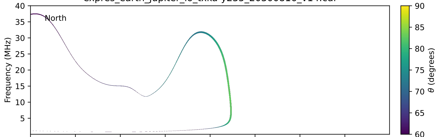
expres_earth_jupiter_io_txka-y235_20300816_v14.cdf
