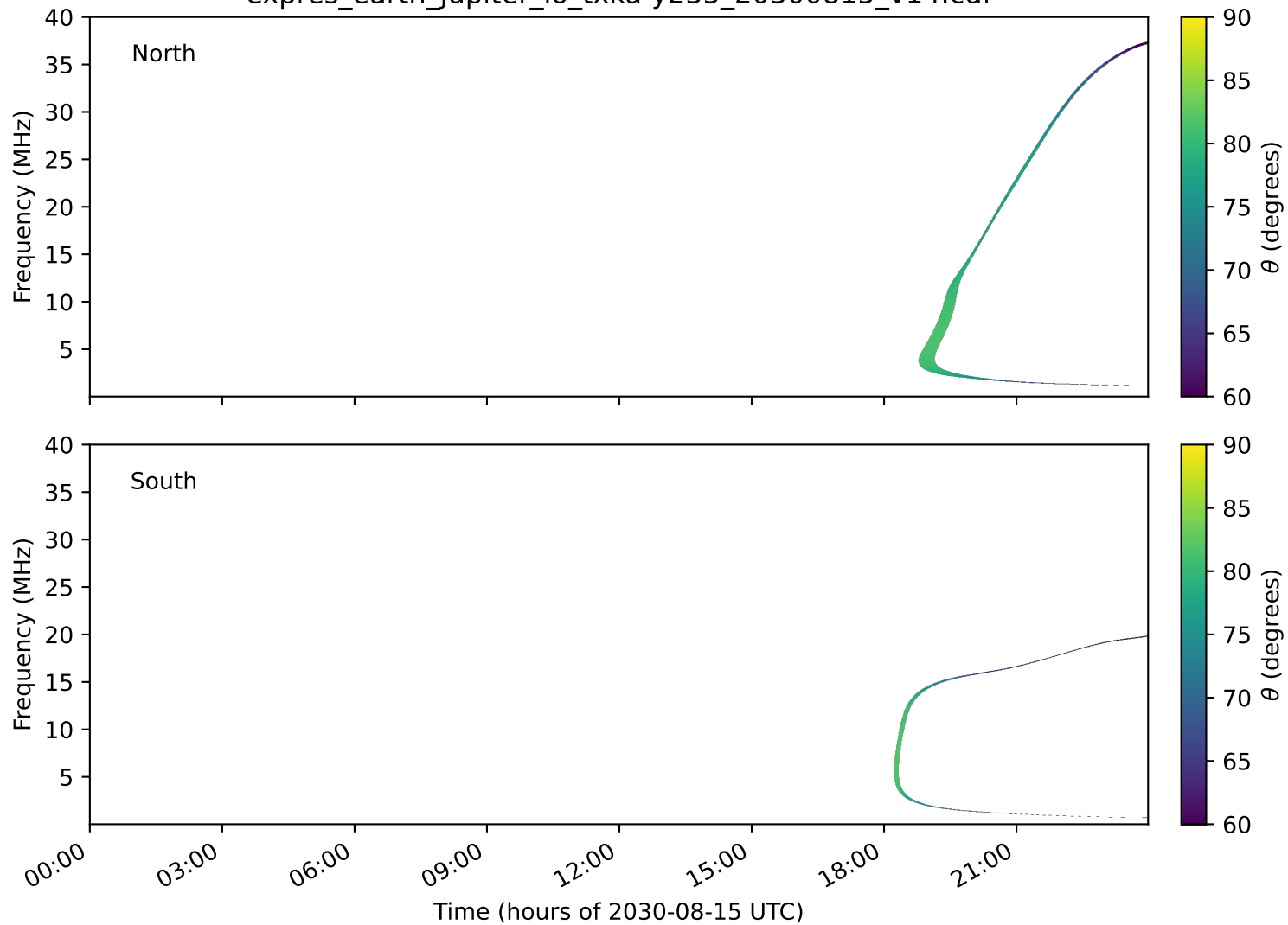
expres_earth_jupiter_io_txka-y235_20300815_v14.cdf
