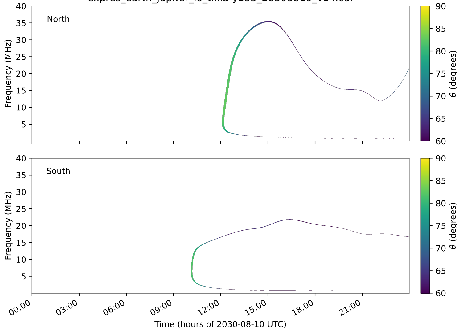
expres_earth_jupiter_io_txka-y235_20300810_v14.cdf
