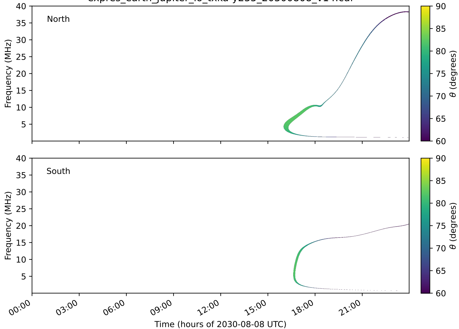
expres_earth_jupiter_io_txka-y235_20300808_v14.cdf
