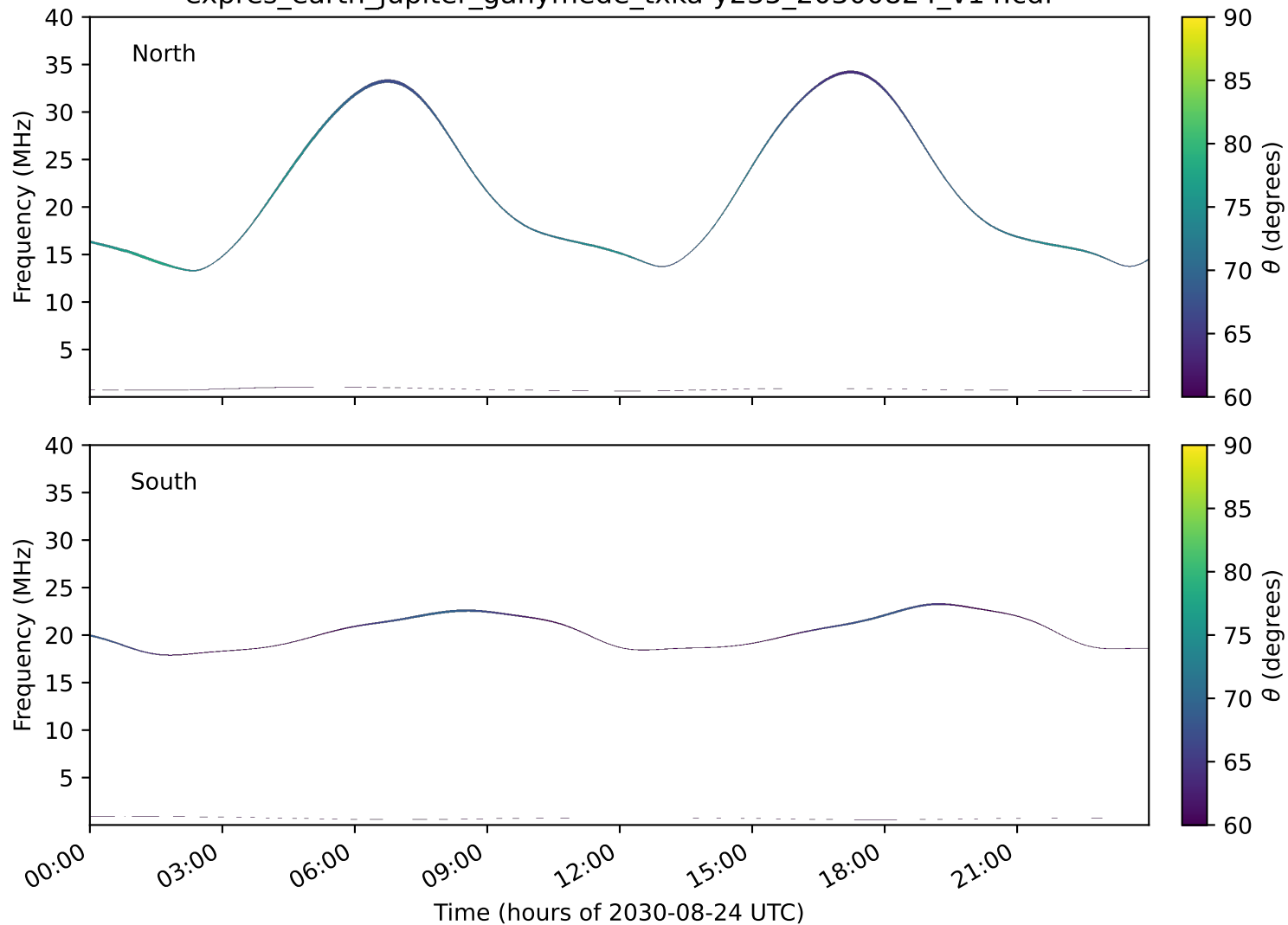
expres_earth_jupiter_ganymede_txka-y235_20300824_v14.cdf
