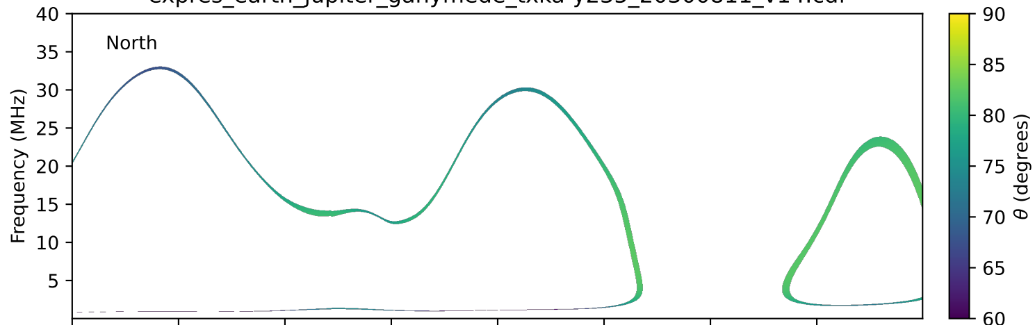
expres_earth_jupiter_ganymede_txka-y235_20300811_v14.cdf
