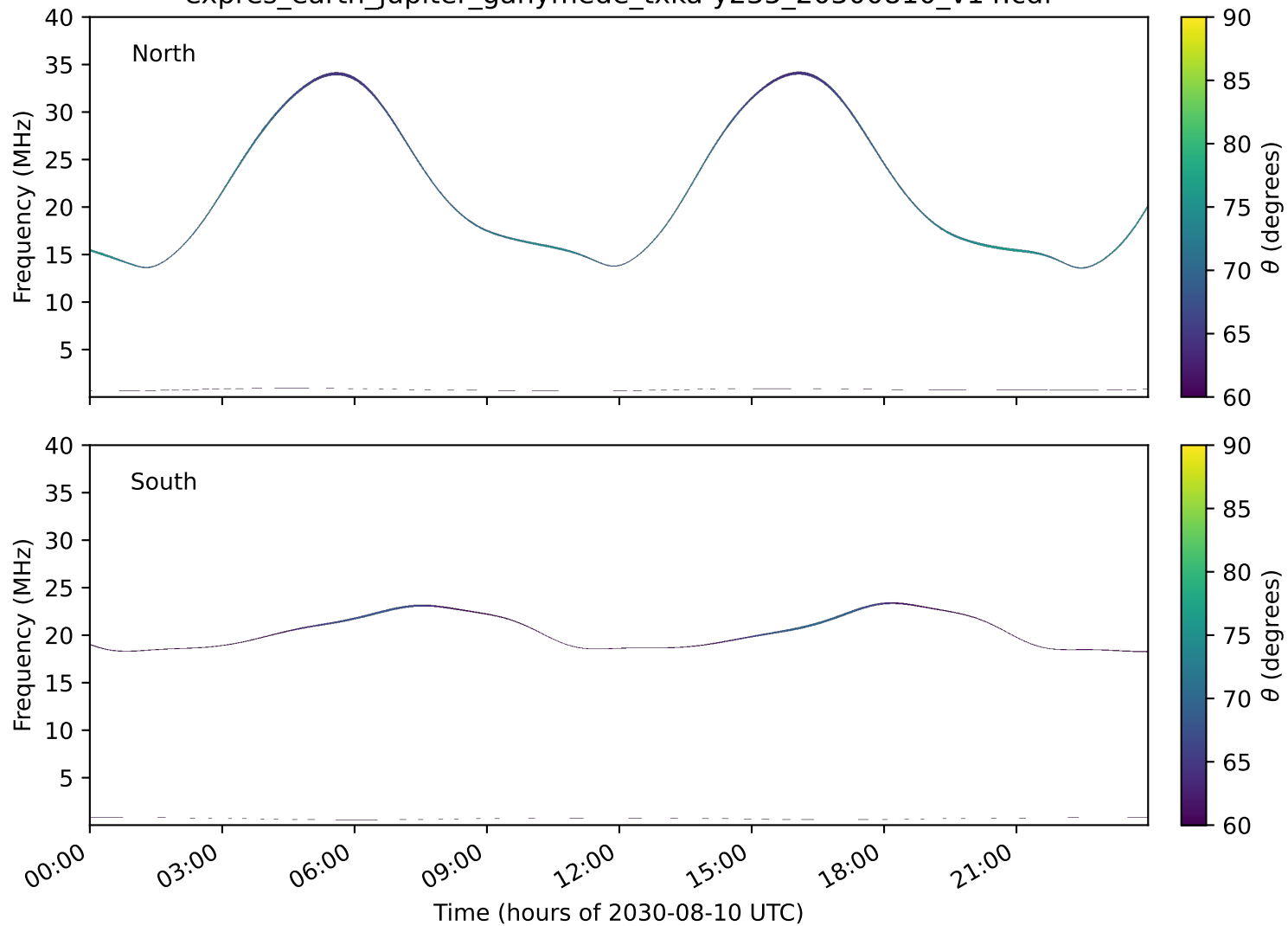
expres_earth_jupiter_ganymede_txka-y235_20300810_v14.cdf
