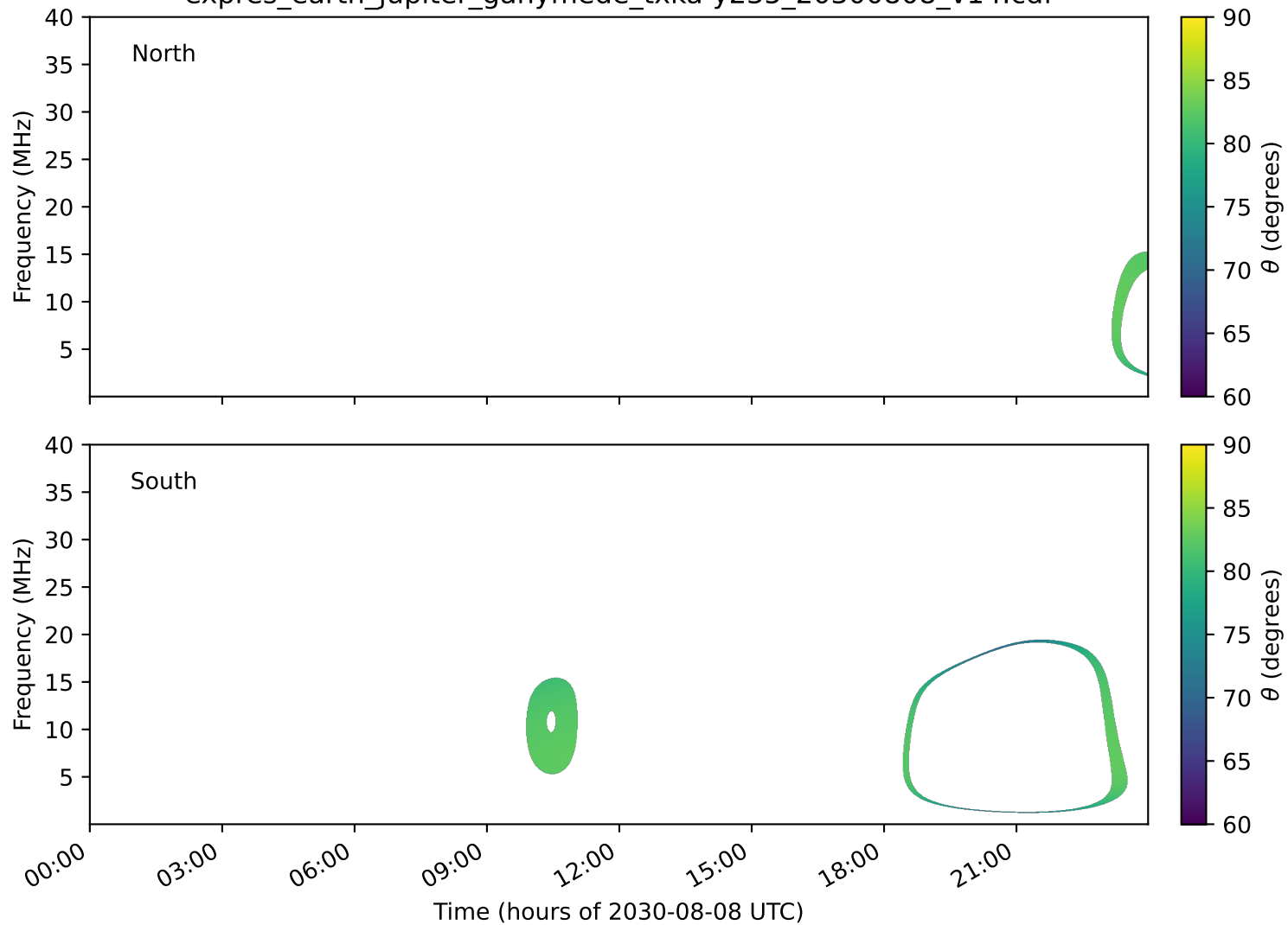
expres_earth_jupiter_ganymede_txka-y235_20300808_v14.cdf
