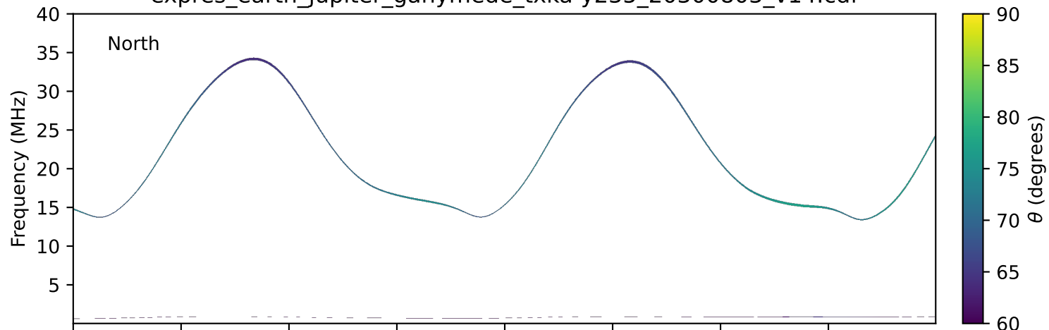
expres_earth_jupiter_ganymede_txka-y235_20300803_v14.cdf
