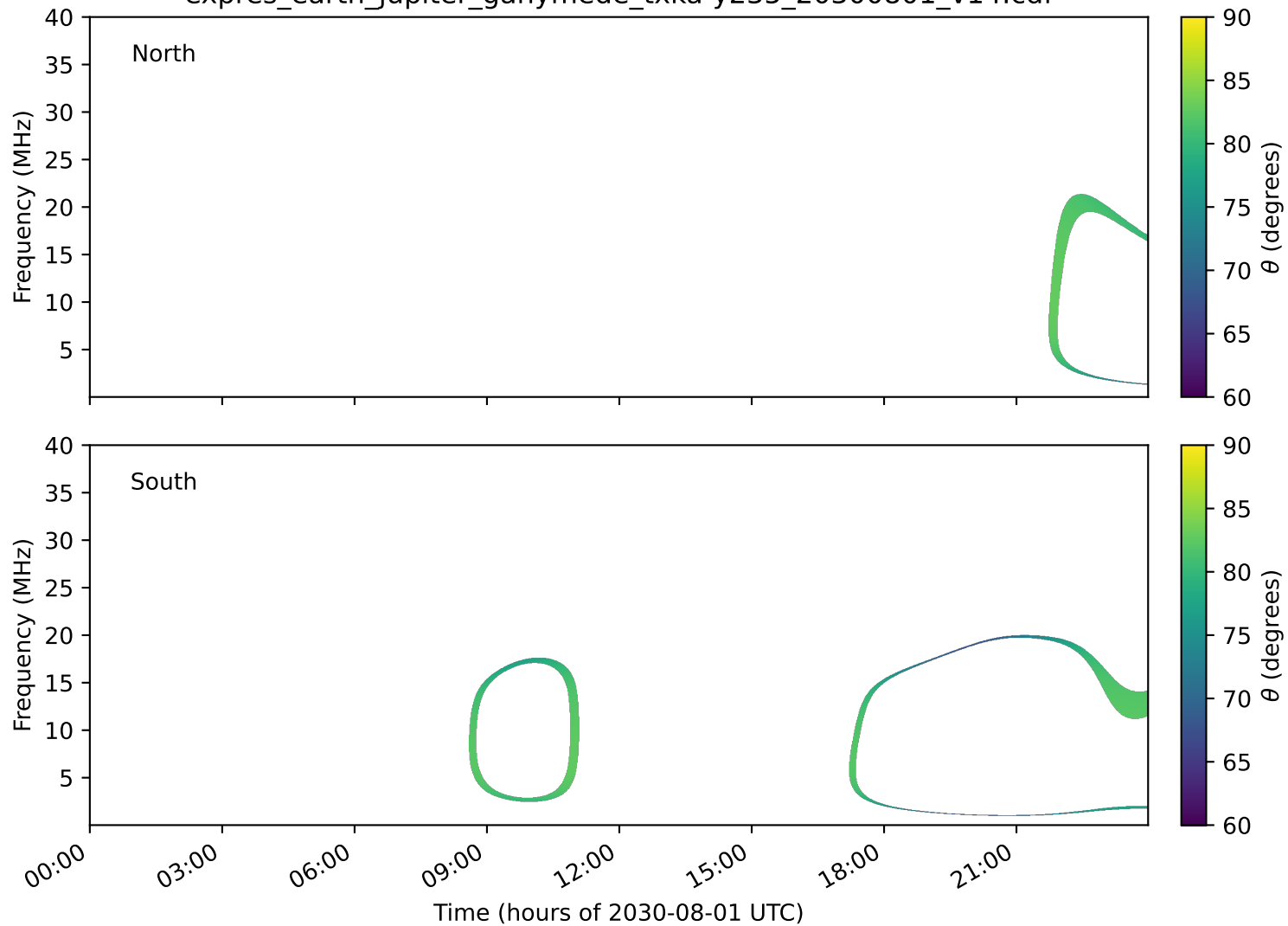
expres_earth_jupiter_ganymede_txka-y235_20300801_v14.cdf
