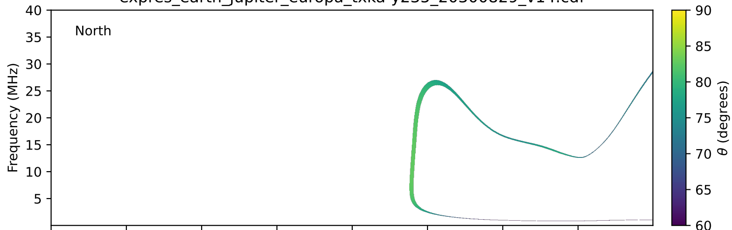
expres_earth_jupiter_europa_txka-y235_20300829_v14.cdf
