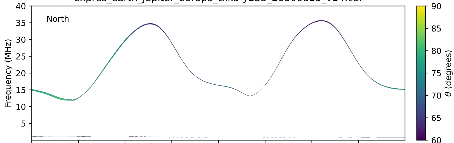
expres_earth_jupiter_europa_txka-y235_20300819_v14.cdf
