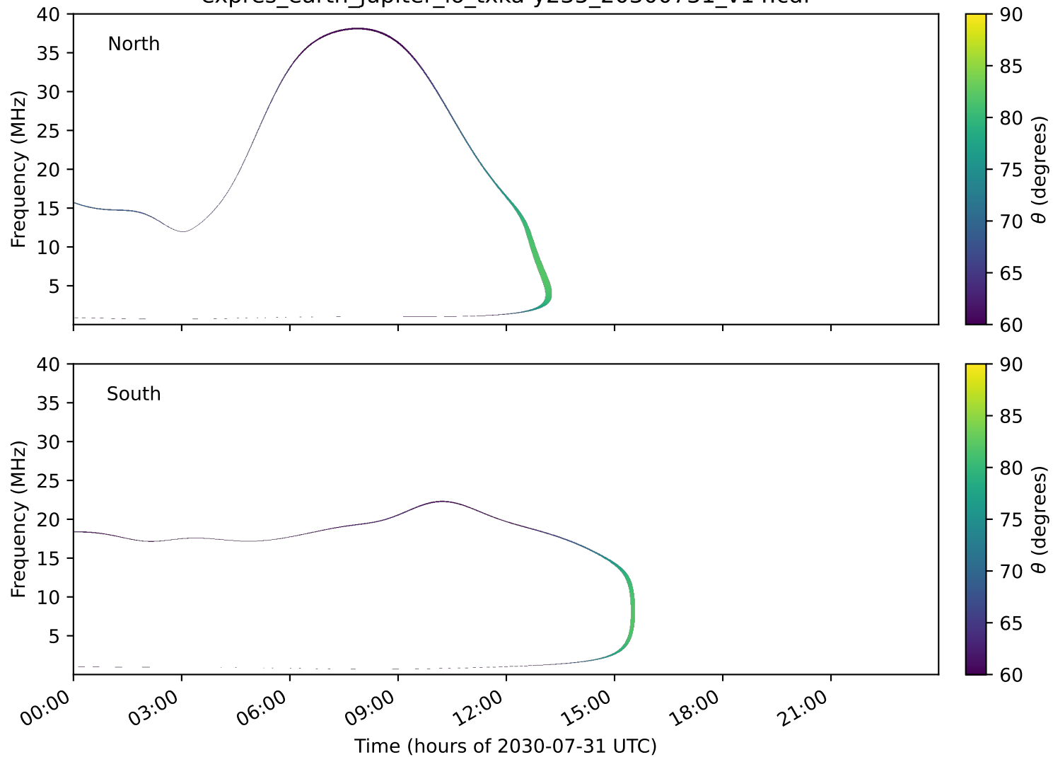
expres_earth_jupiter_io_txka-y235_20300731_v14.cdf
