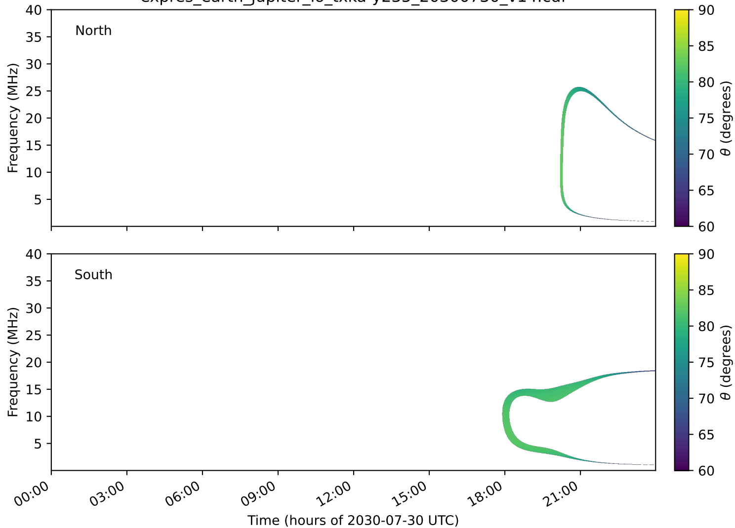
expres_earth_jupiter_io_txka-y235_20300730_v14.cdf
