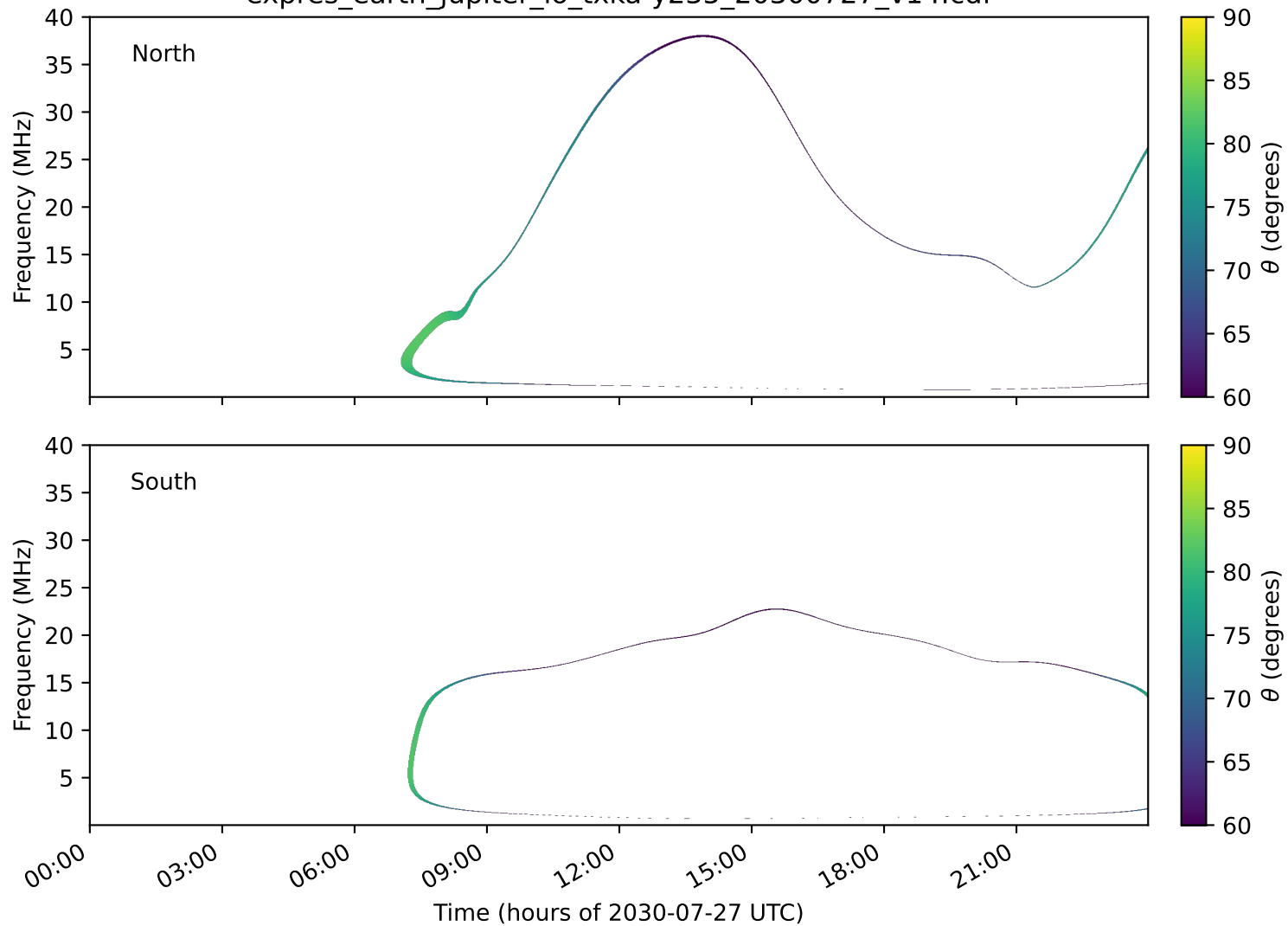
expres_earth_jupiter_io_txka-y235_20300727_v14.cdf
