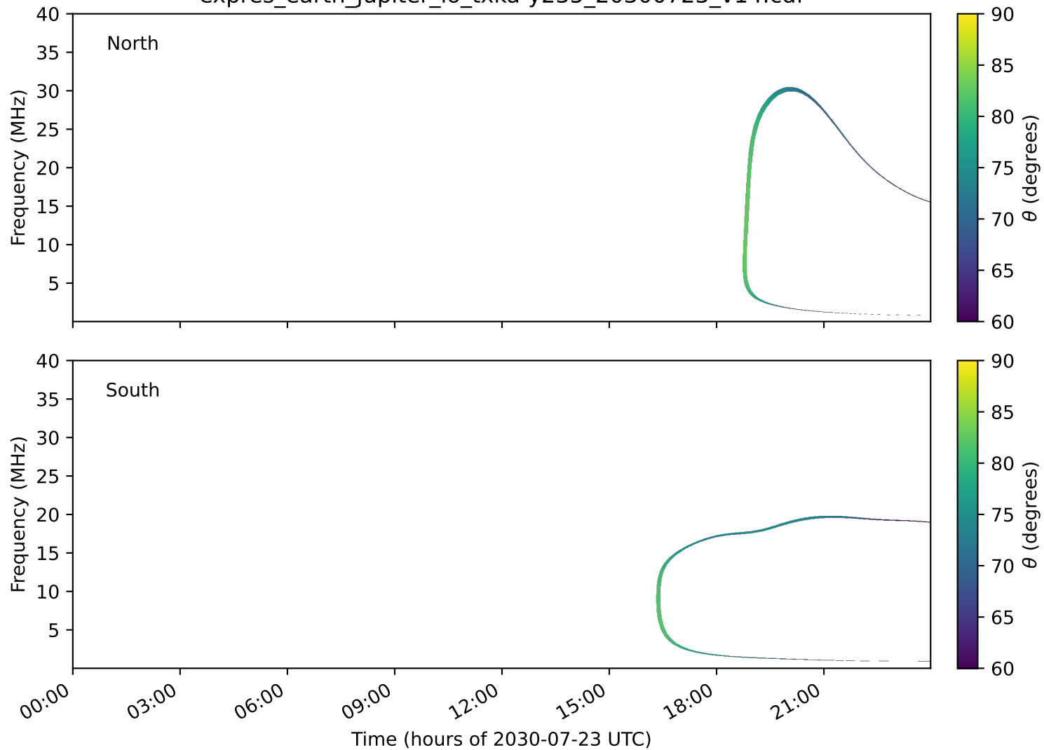
expres_earth_jupiter_io_txka-y235_20300723_v14.cdf
