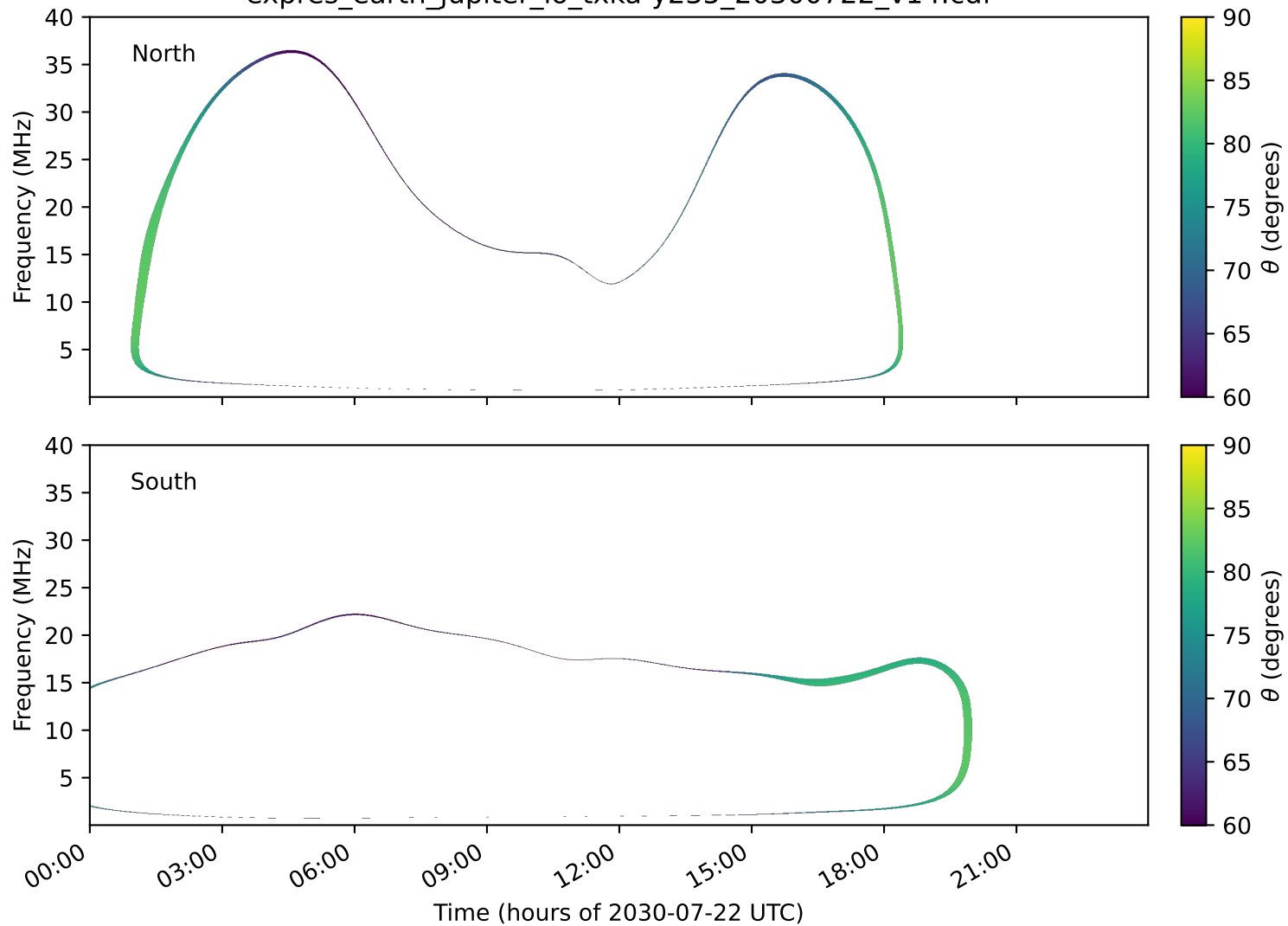
expres_earth_jupiter_io_txka-y235_20300722_v14.cdf
