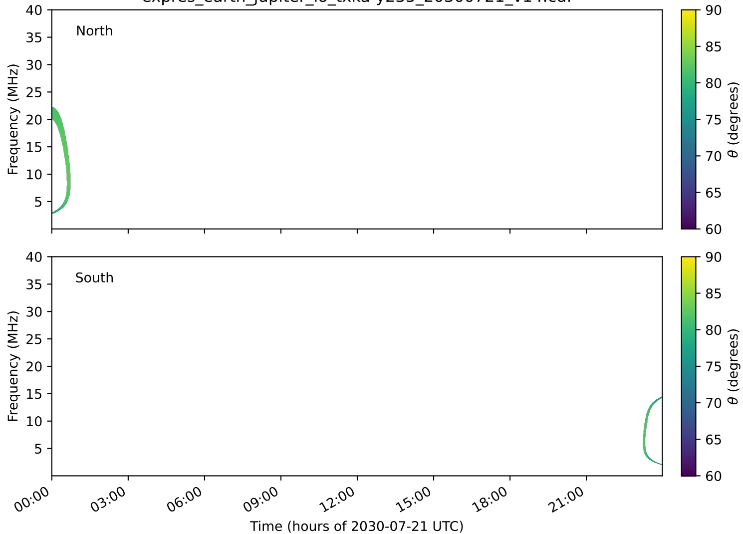
expres_earth_jupiter_io_txka-y235_20300721_v14.cdf
