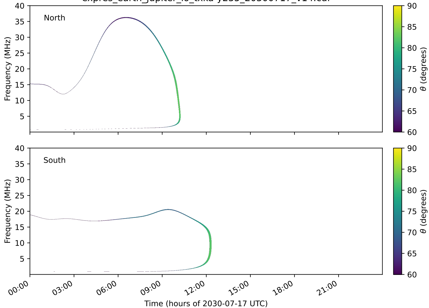
expres_earth_jupiter_io_txka-y235_20300717_v14.cdf
