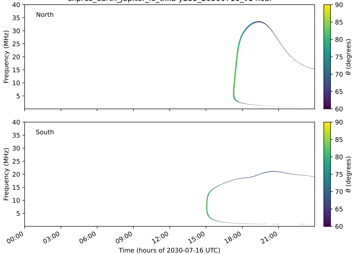
expres_earth_jupiter_io_txka-y235_20300716_v14.cdf
