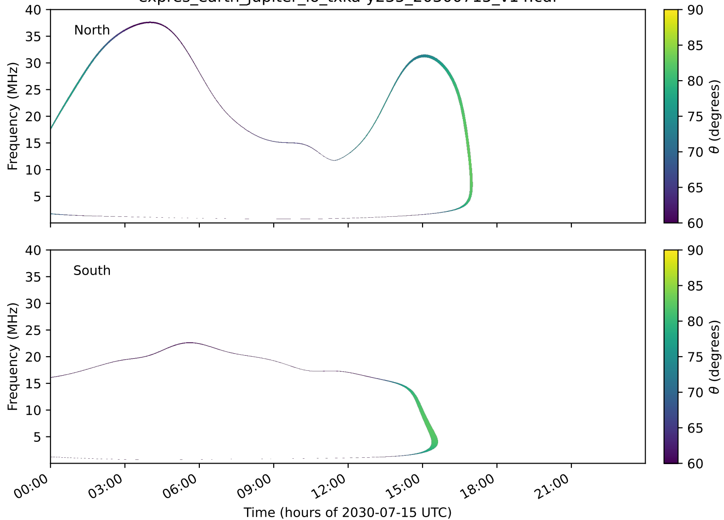
expres_earth_jupiter_io_txka-y235_20300715_v14.cdf
