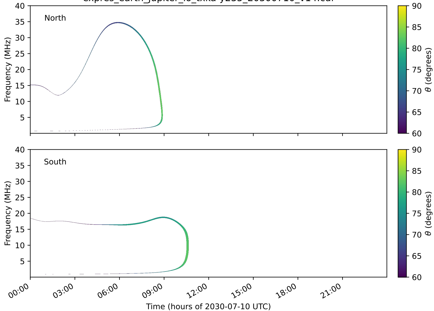
expres_earth_jupiter_io_txka-y235_20300710_v14.cdf
