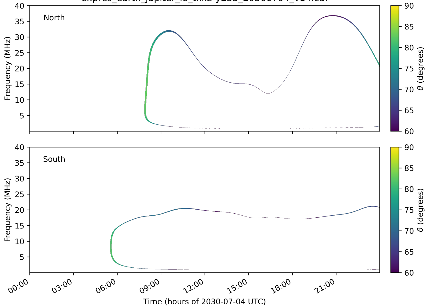
expres_earth_jupiter_io_txka-y235_20300704_v14.cdf
