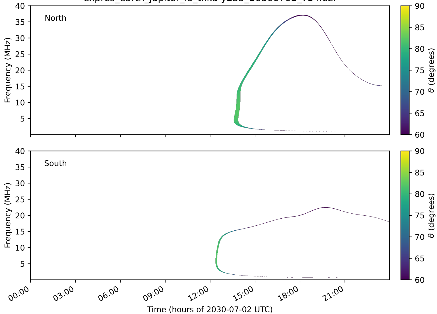
expres_earth_jupiter_io_txka-y235_20300702_v14.cdf
