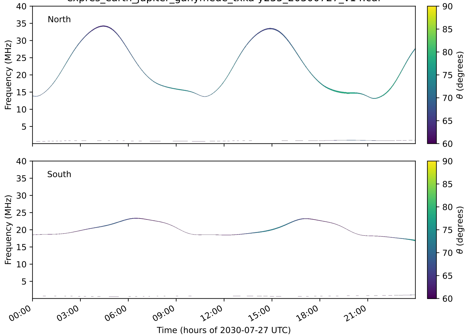
expres_earth_jupiter_ganymede_txka-y235_20300727_v14.cdf
