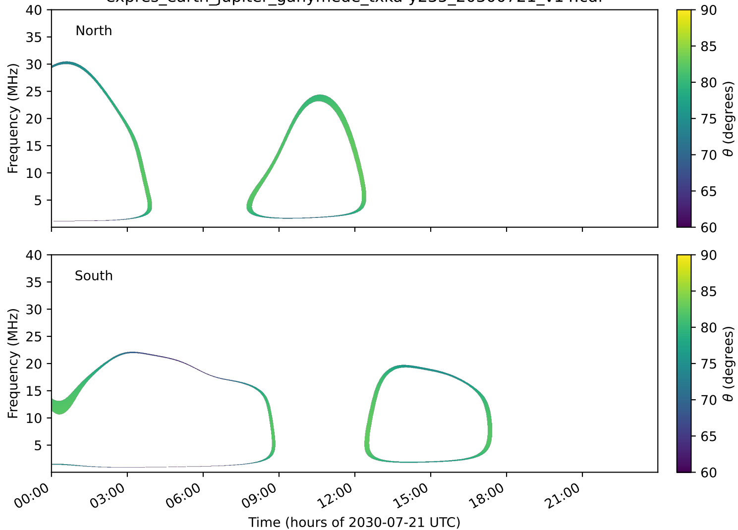
expres_earth_jupiter_ganymede_txka-y235_20300721_v14.cdf
