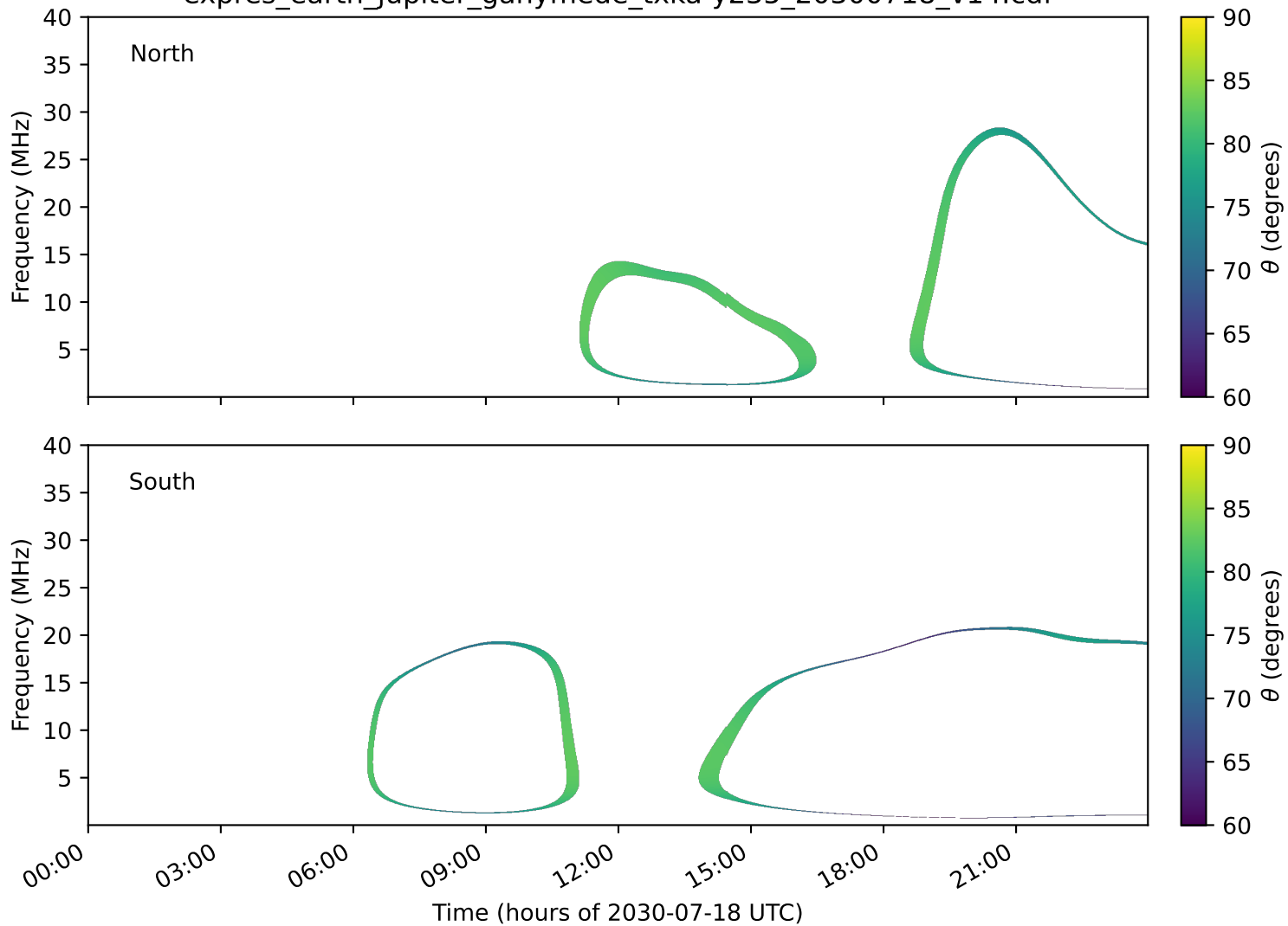
expres_earth_jupiter_ganymede_txka-y235_20300718_v14.cdf
