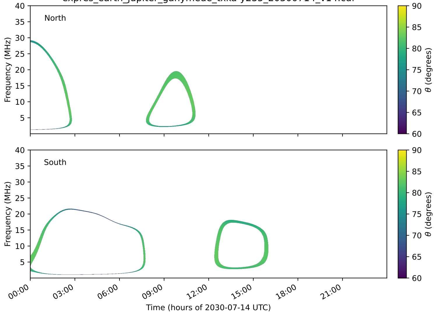
expres_earth_jupiter_ganymede_txka-y235_20300714_v14.cdf
