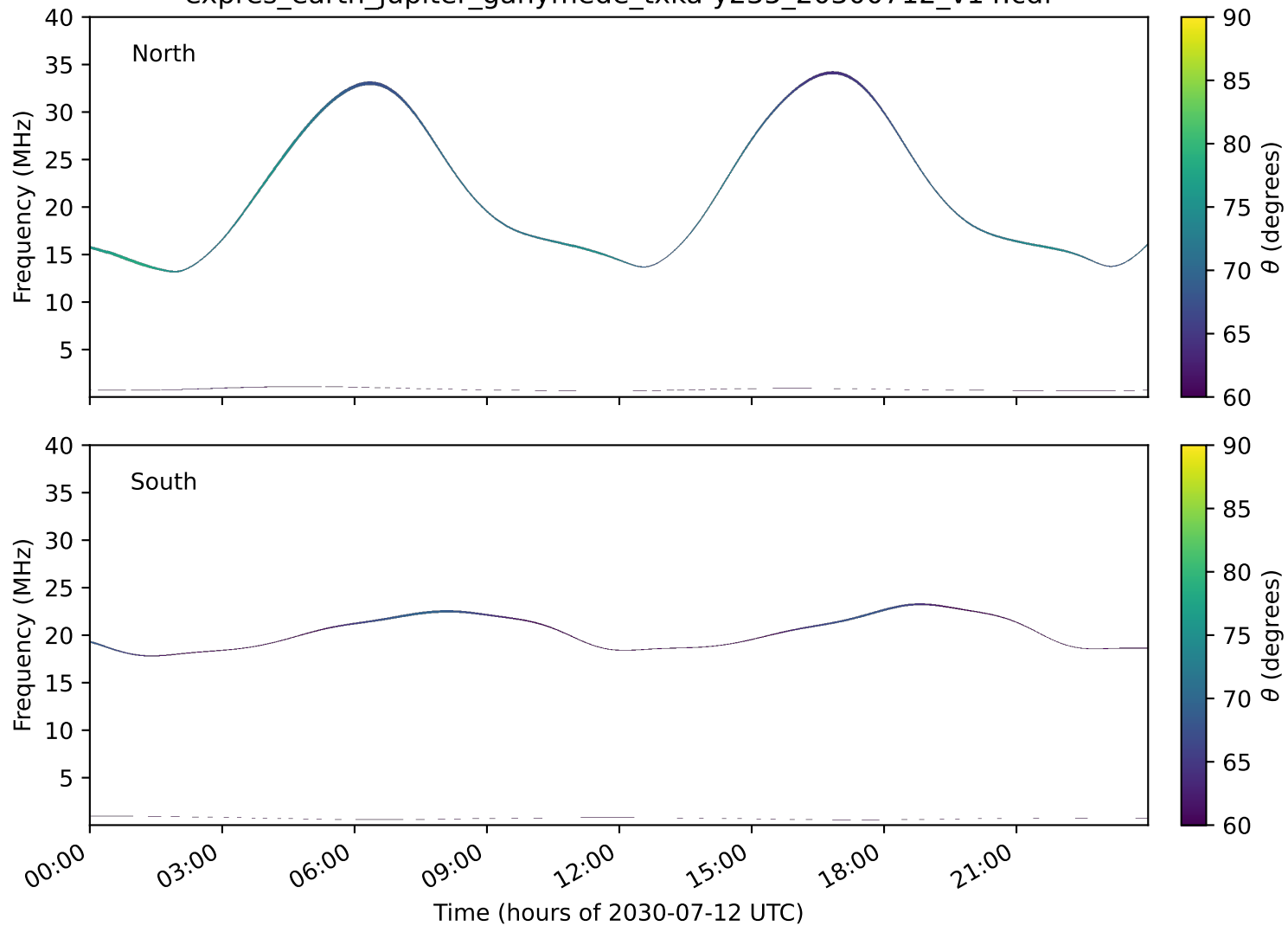
expres_earth_jupiter_ganymede_txka-y235_20300712_v14.cdf
