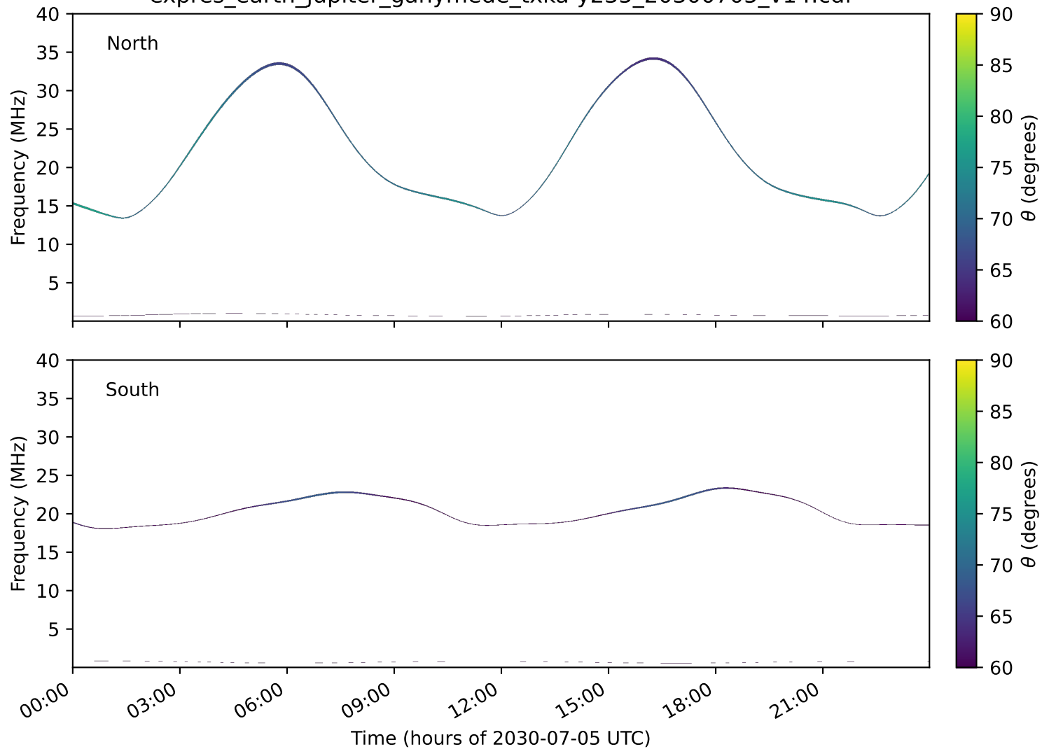
expres_earth_jupiter_ganymede_txka-y235_20300705_v14.cdf
