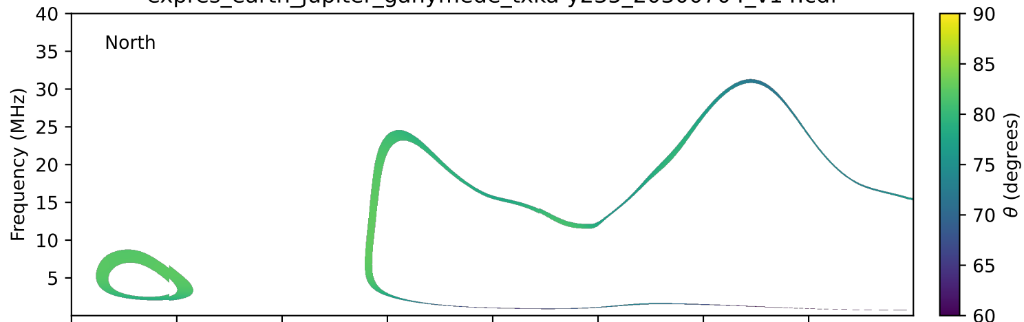
expres_earth_jupiter_ganymede_txka-y235_20300704_v14.cdf
