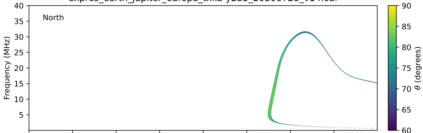
expres_earth_jupiter_europa_txka-y235_20300728_v14.cdf
